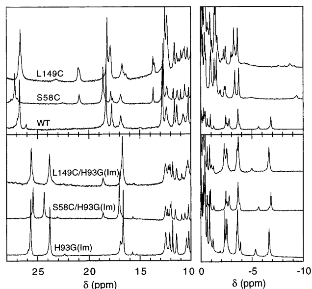
FIGURE 4: ^1\text{H} NMR spectra for the met CN bound form of TFA-labeled, proximal and distal cysteine mutants. (Upper panels) Proximal single mutant L149C, distal single mutant S58C, and wild-type. (Lower panels) Proximal double mutant L149C/H93G(Im), distal single mutant S58C/H93G(Im), and H93G(Im). All spectra were collected as 512 scans of 8 K points with a spectral window of 25 000 Hz.
